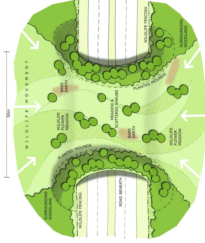
Figure 2: Example sketch of a Wildlife Bridge
